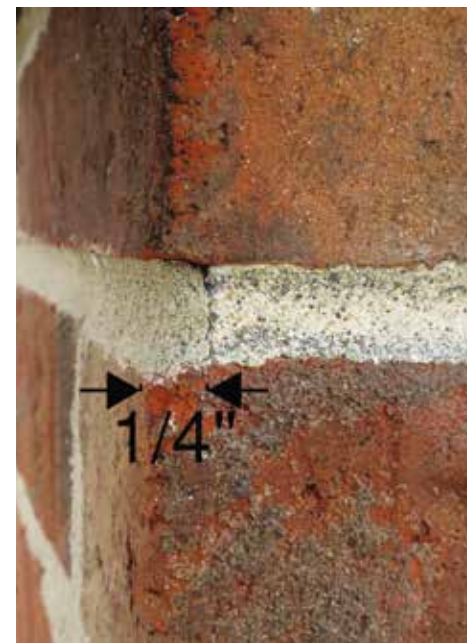
Figure 7. Mortar joint repointing to an insufficient depth of approximately \frac{1}{4} in. (6.4 mm).
